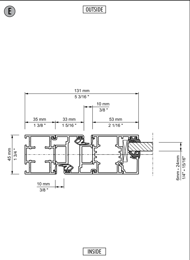
Description: Horizontal-Section, blind frame - panel closing section / inside folding System: SF45 Detail-No.: SF45-101
