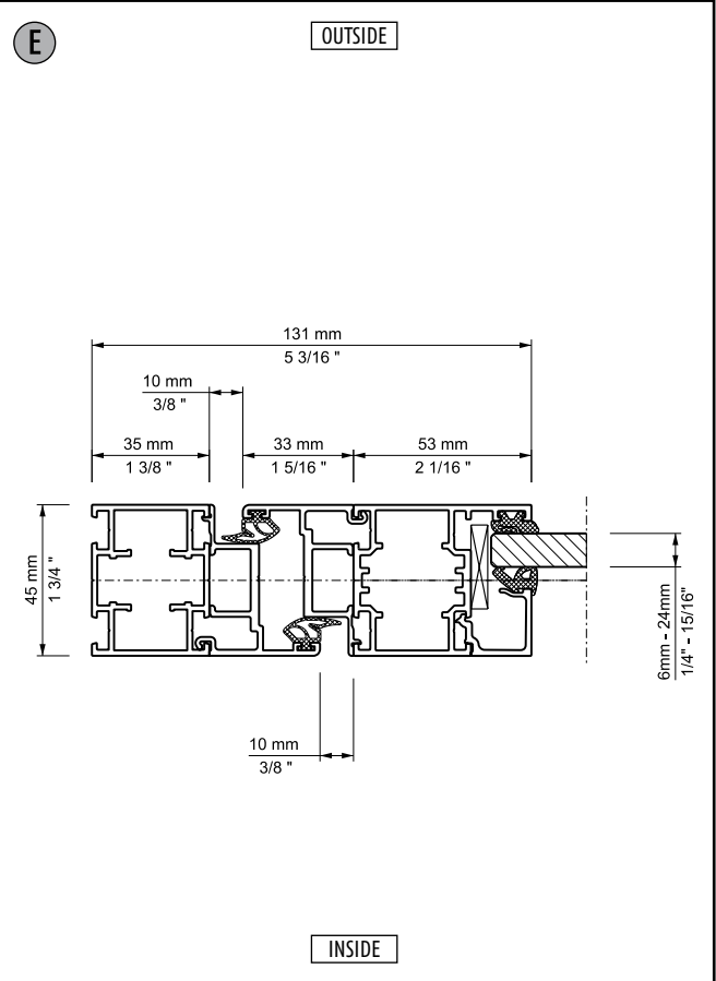
Description: Horizontal-Section, blind frame - panel closing section / outside folding System: SF45 Detail-No.: SF45-102
