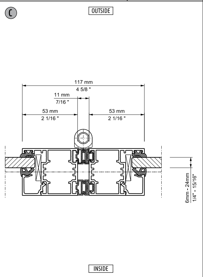
Description: Horizontal-Section, panel - panel / hinge outside System: SF45 Detail-No.: SF45-103
