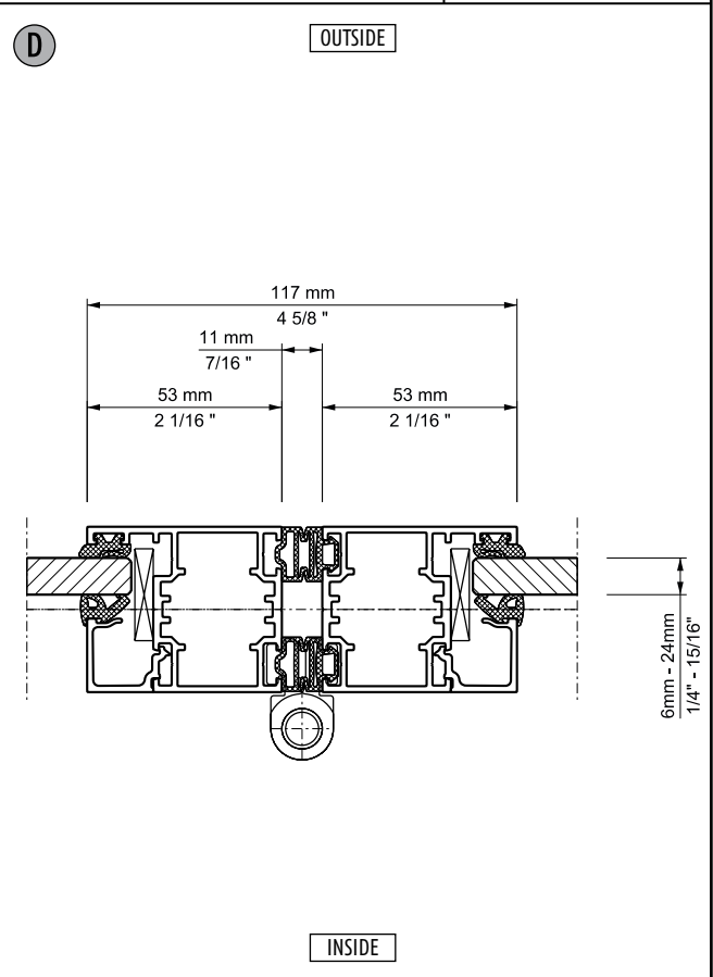
Description: Horizontal-Section, panel - panel / hinge inside System: SF45 Detail-No.: SF45-104
